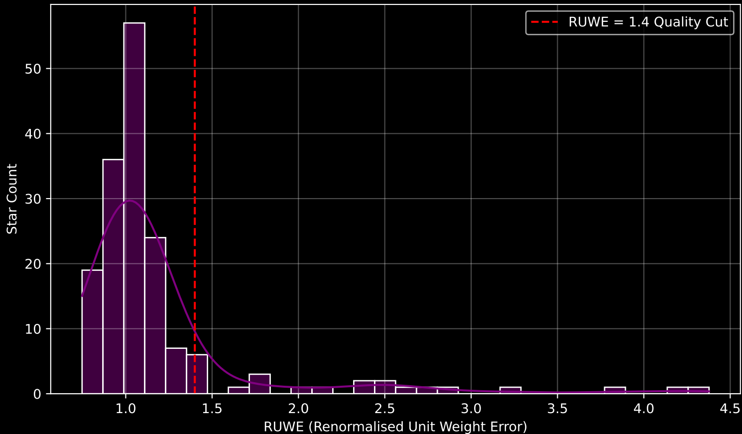
GAPOGEE DR17 Field [286-29-O_TESS] RUWE Distribution (n= 166)
