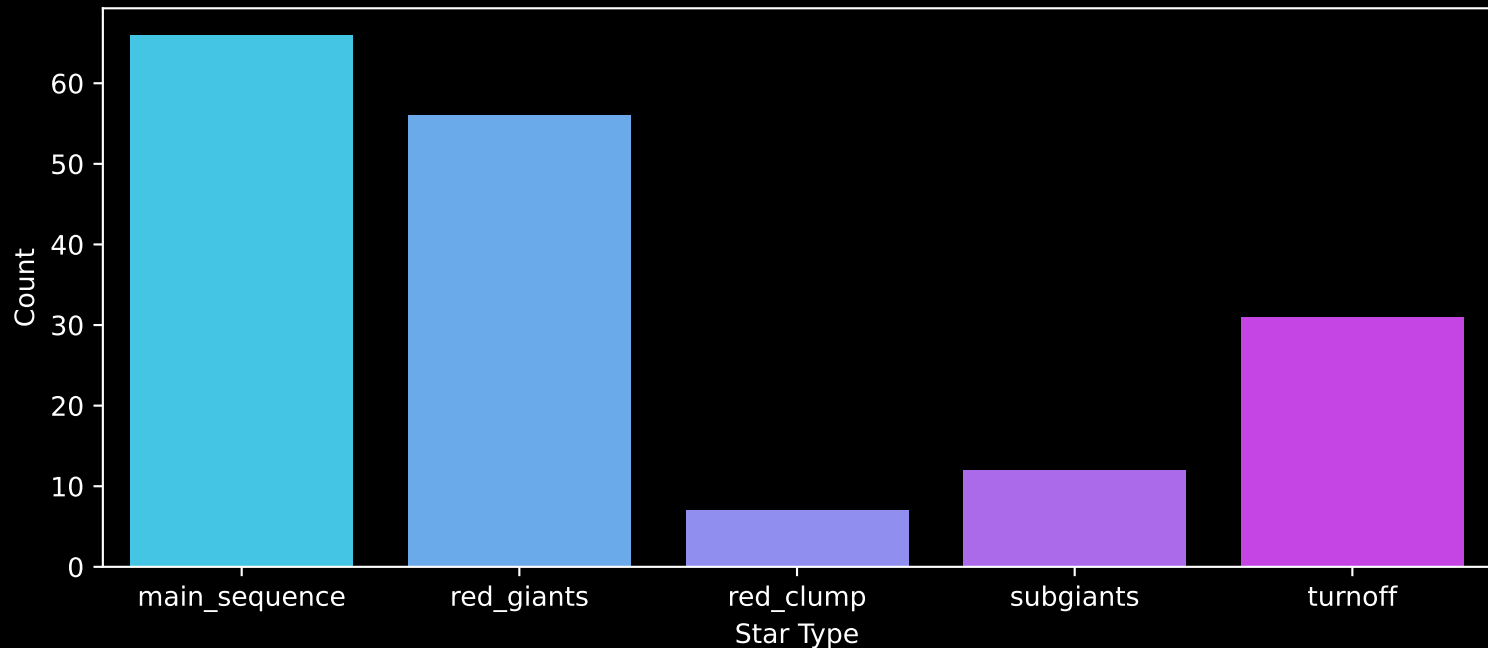
APOGEE DR17 Field: [286-29-O_TESS] Count plot of Star Type
