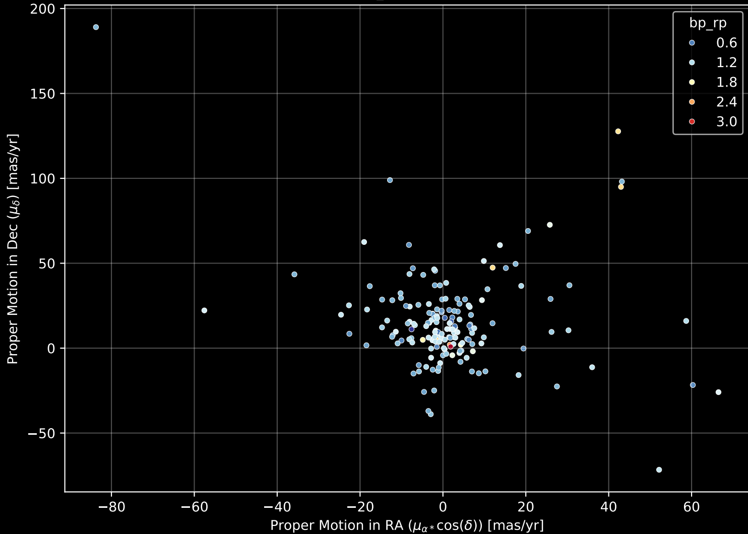
APOGEE DR17 Field: [286-29-O_TESS] Proper Motion Diagram (n= 172)
