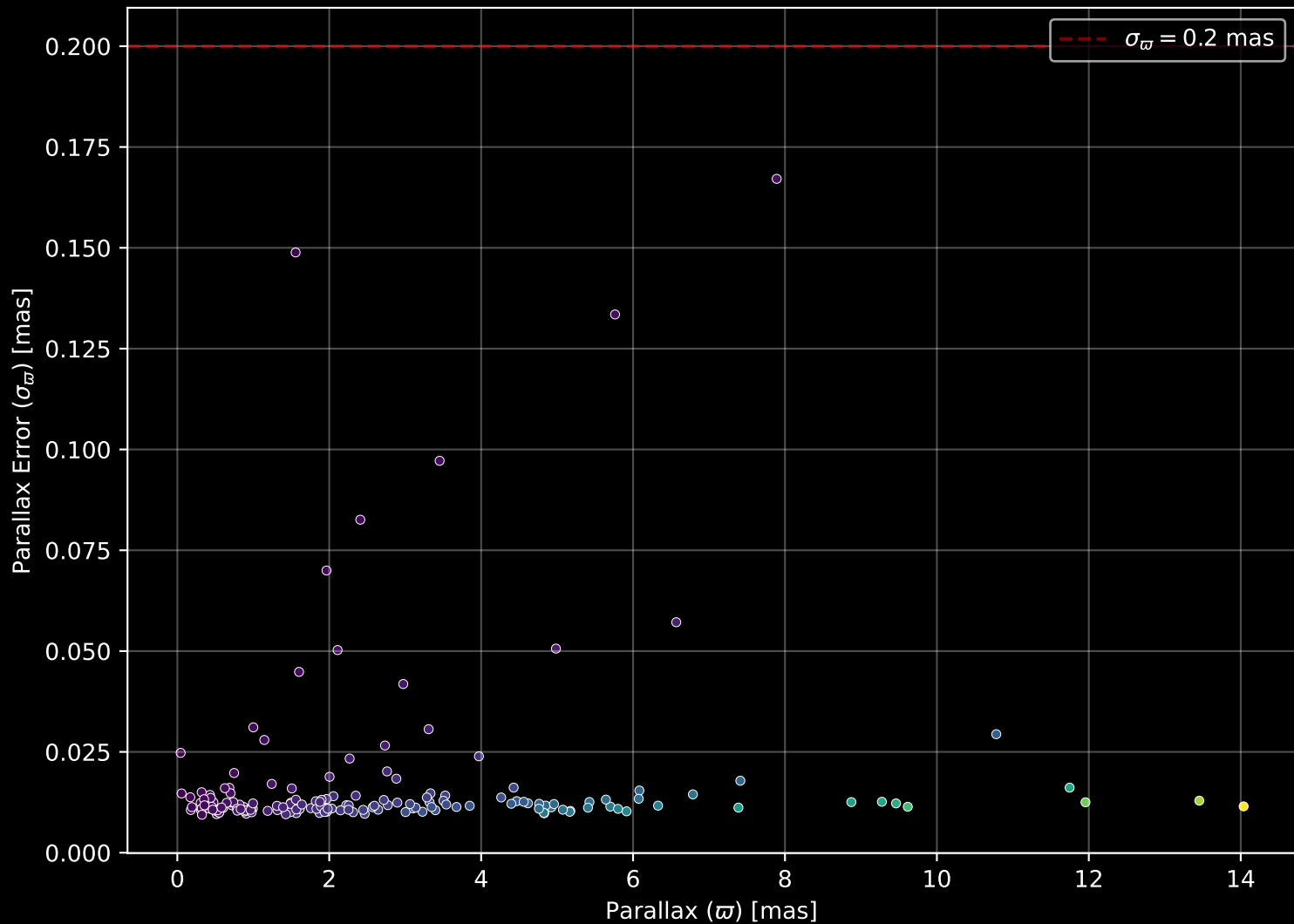
APOGEE DR17 Field: [286-29-O_TESS] Parallax Quality (n= 172)
