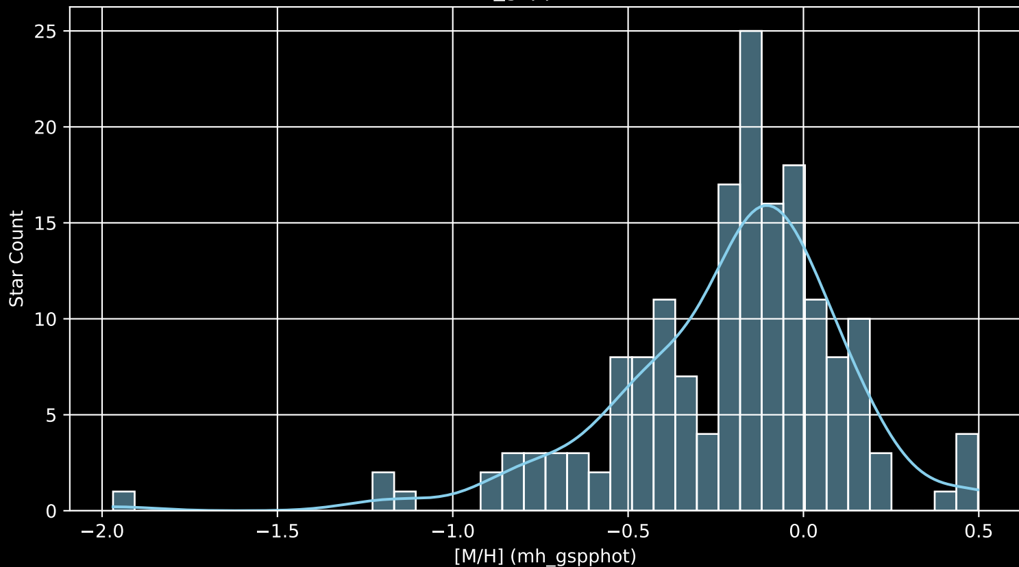
APOGEE DR17 Field: [286-29-O_TESS [M/H] (mh_gspphot) (n= 171)
